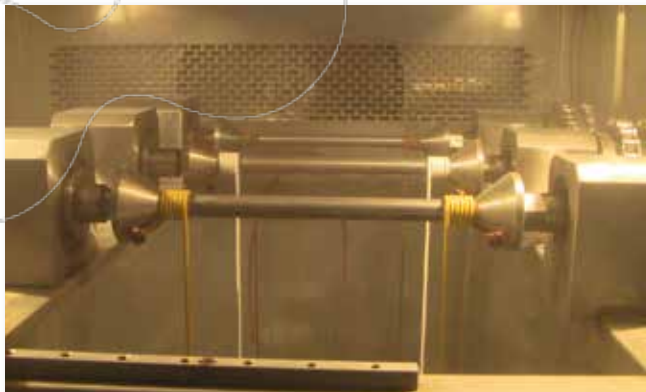
Cable samples in a cyclic strength test.
