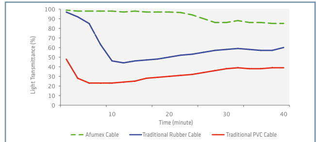
LS0H. Smoke density graphs for rubber and PVC.
