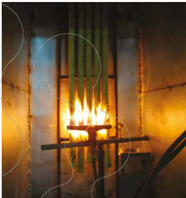
Cable samples in the harnessed cable burning test.
