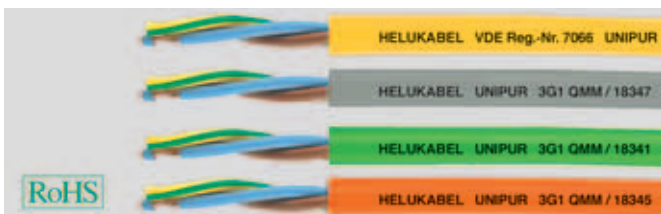
Part no. 18120
