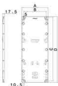
Mounting plates
