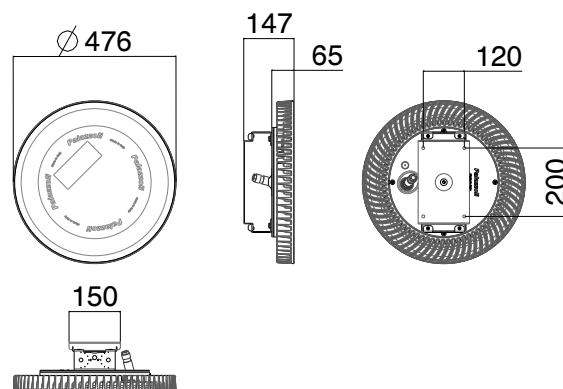
Ceiling mounting
