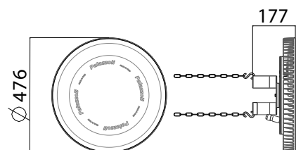
Adjustable double chain suspension
