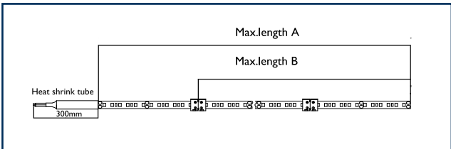
A: Maximum length of LED tape in case tape starts with heat shrink tube (soldered wires to LED tape).
